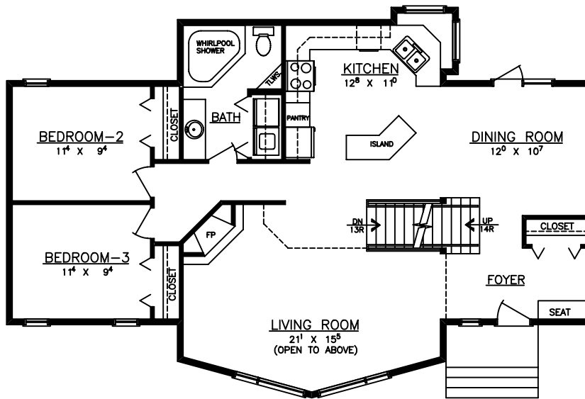
MAIN FLOOR AREA = 1179 S.F.
